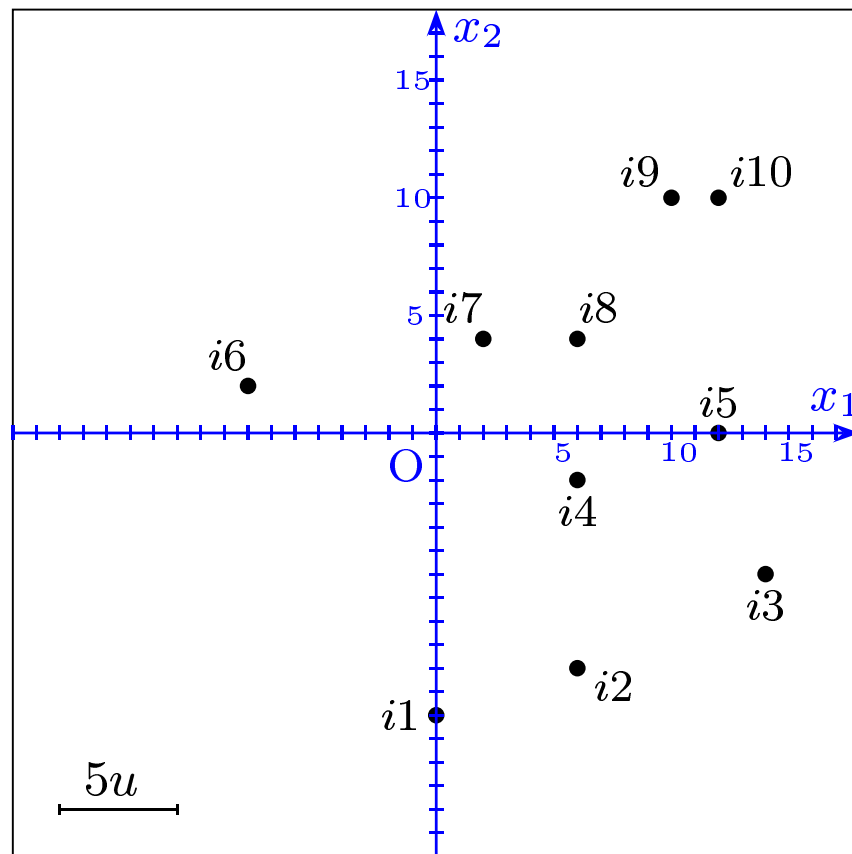
Figure 1bis: Cloud with origin-point (point \textcolor{blue}{O} ) and initial axes
