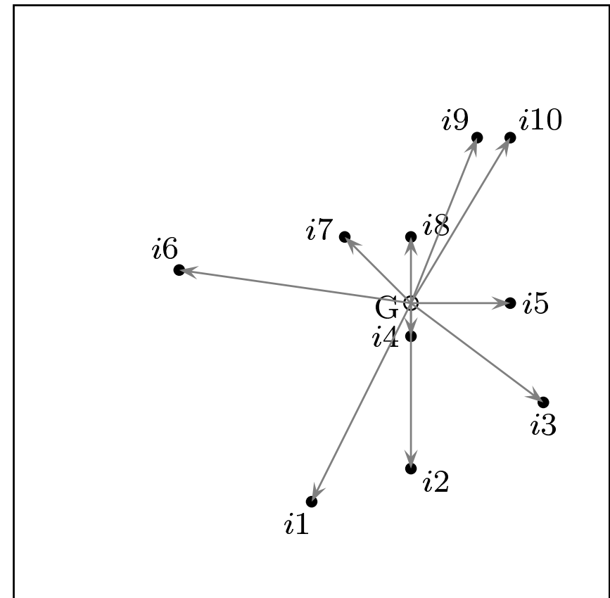
Figure 2: Mean point and Barycentric Property
